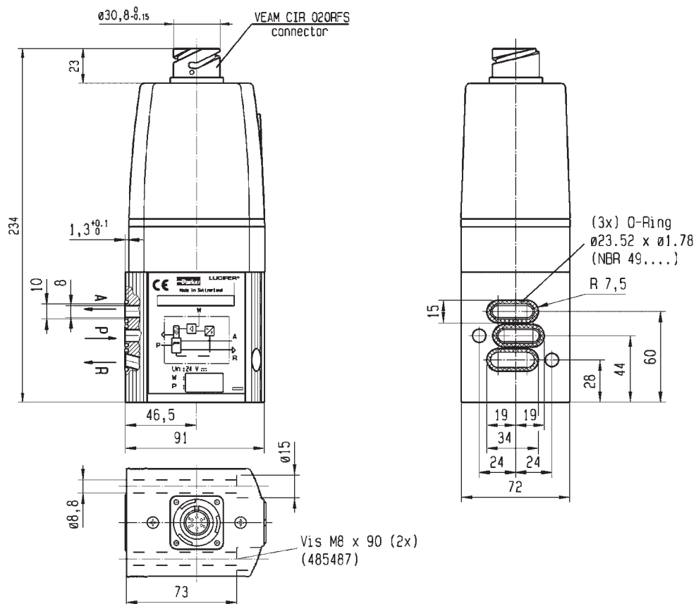
EPP3 with ISO 3 flange connection
