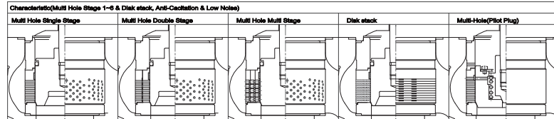
ACMB, LNM(Single Seated Cage Guide - Under The Wep & Over The Wep)
