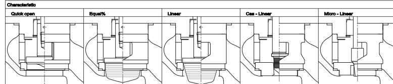
ACC TYPE(Single Seated Cage Guide - Under & Over The Wep)
